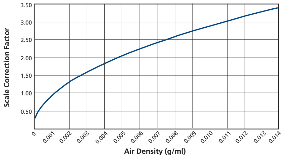
Air Density vs. Flow Factor
